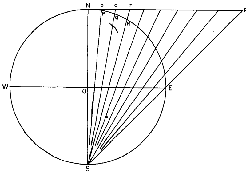
FIG. 21.—Determination of radii for stereographic polar projection.
