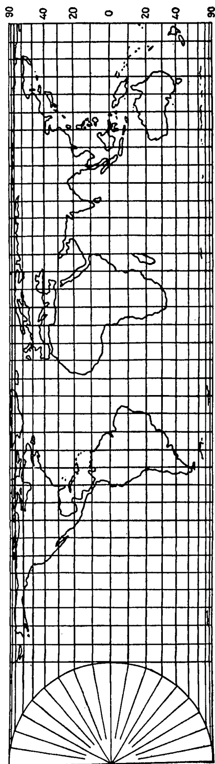
FIG. 16.—Cylindrical equal-area projection.
