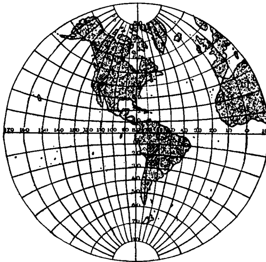
FIG. 30.—Stereographic projection of the Western Hemisphere.
