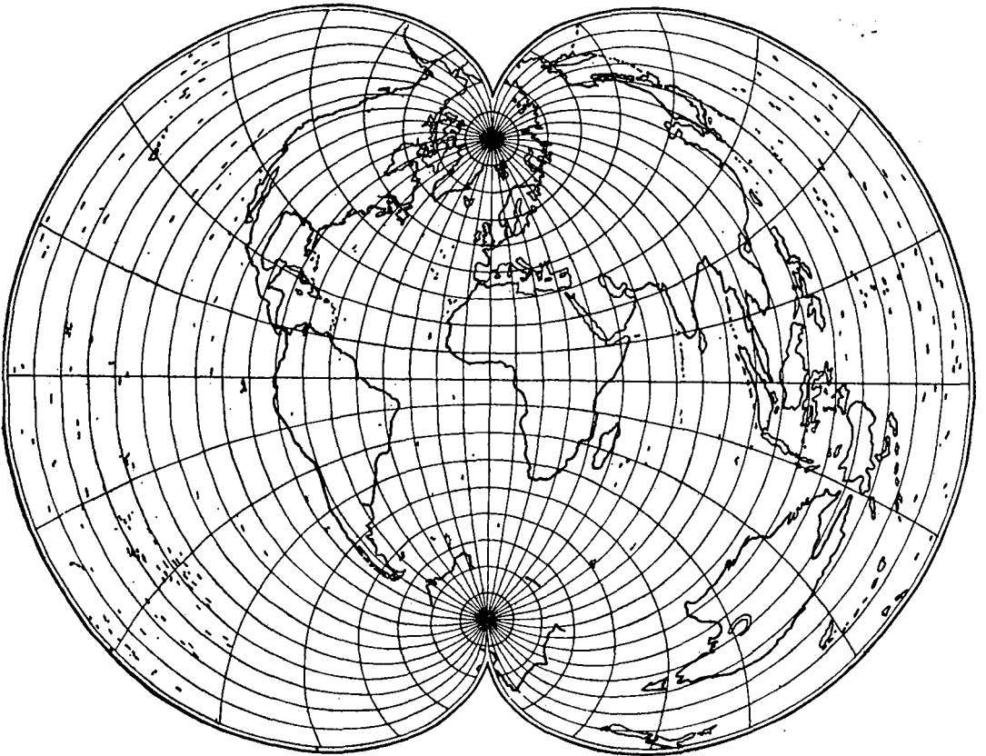
FIG. 47.—Polyconic development of the sphere.
