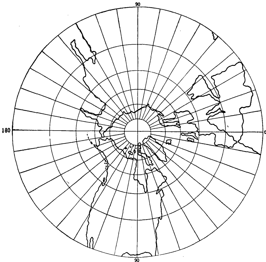
FIG. 24.—Gnomonic polar projection.
